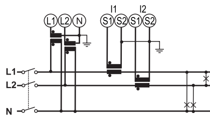
Fig. 16 Two-phase system (3-wire), 2 CT and 2 VT/PT.
